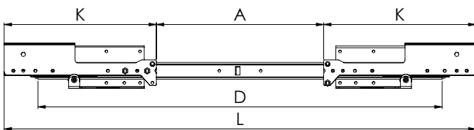
Asansörlü Masa Rayı / Table Rail With Lift
